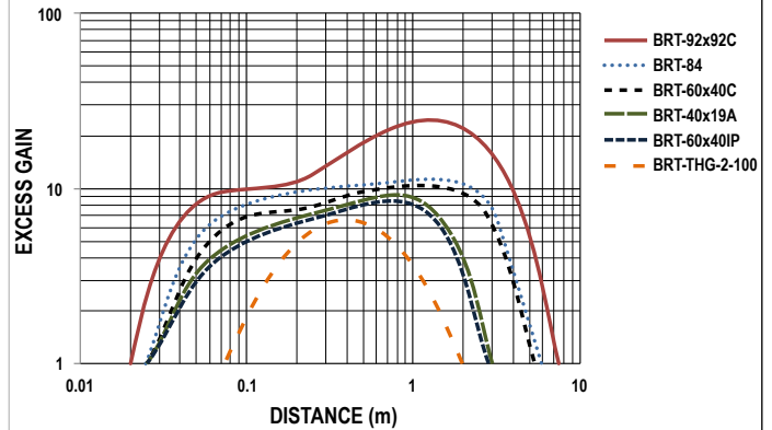
Excess Gain
