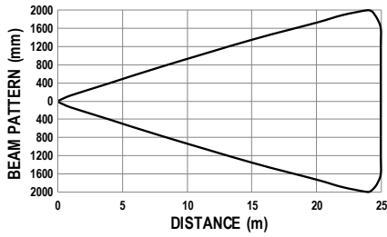
Beam Pattern
