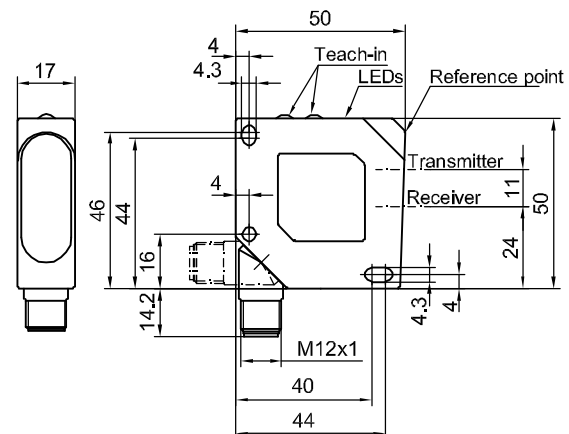
Dimensional drawing
