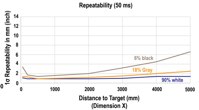
Figure 31. Repeatability for 50 ms Response Time
