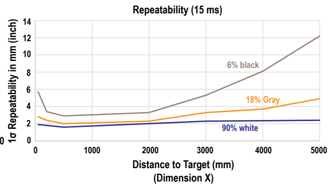
Figure 33. Repeatability for 15 ms Response Time
