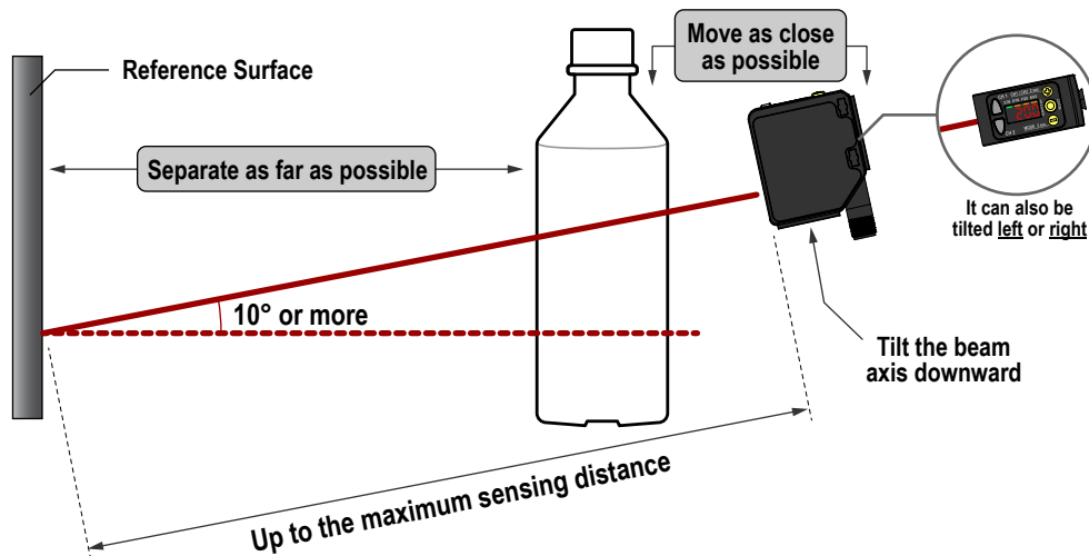
Figure 38. Common problems and solutions for detecting clear objects
