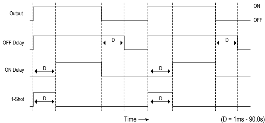
Figure 19. Output Timing Delays
