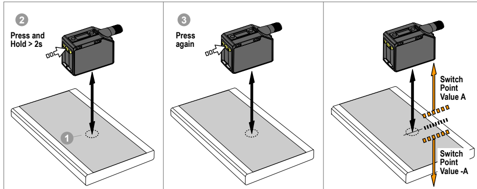
Figure 24. One-Point Window (Foreground Suppression)
