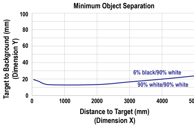
Figure 28. Minimum Object Separation for 250 ms Response Time
