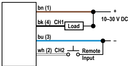
Figure 14. Channel 1 = NPN Output, Channel 2 = NPN Remote Input
