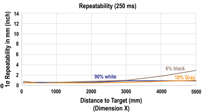
Figure 29. Repeatability for 250 ms Response Time
