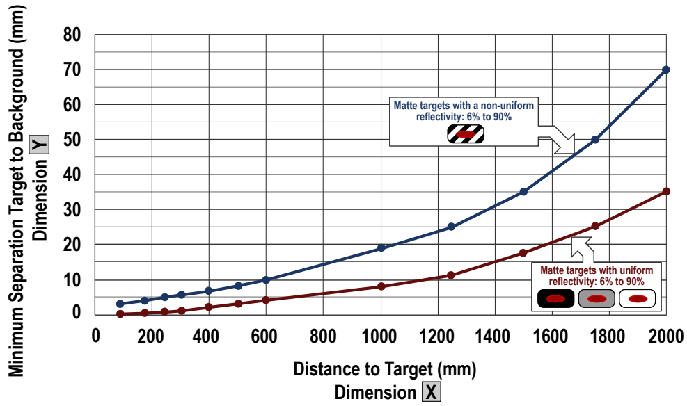
Figure 27. Performance for the 2000 mm Models
