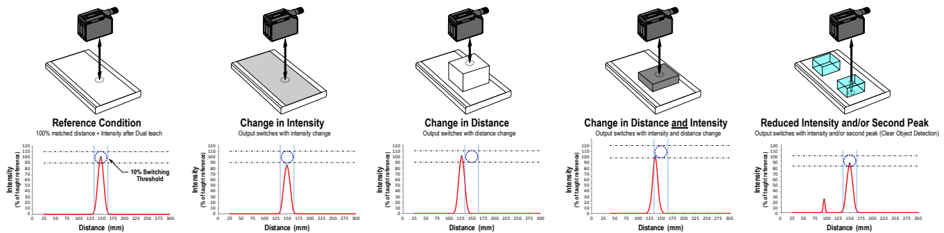
Figure 36. Dual Mode Example
