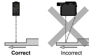
Figure 7. Orientation for a height difference
