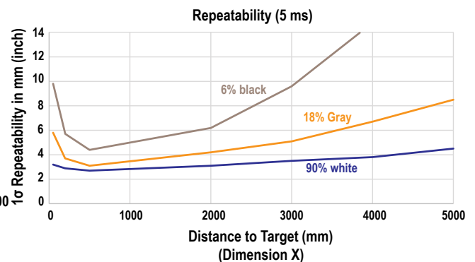
Figure 35. Repeatability for 5 ms Response Time
