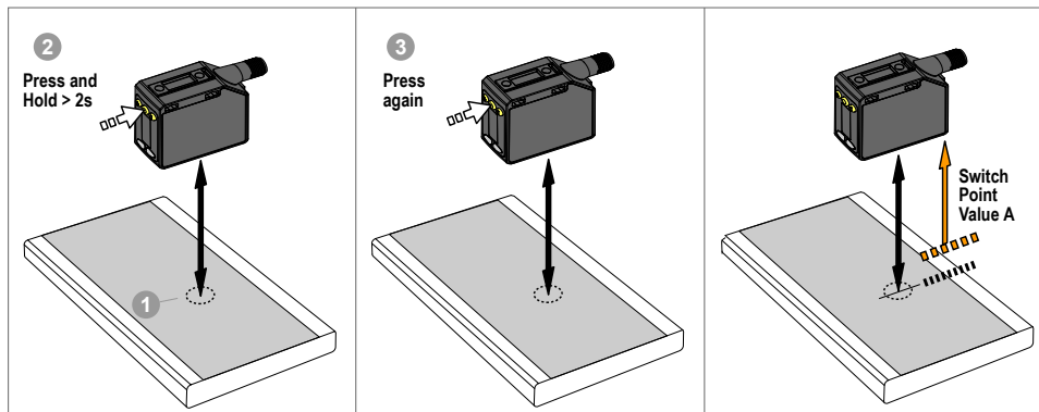
Figure 25. One-Point Background Suppression
