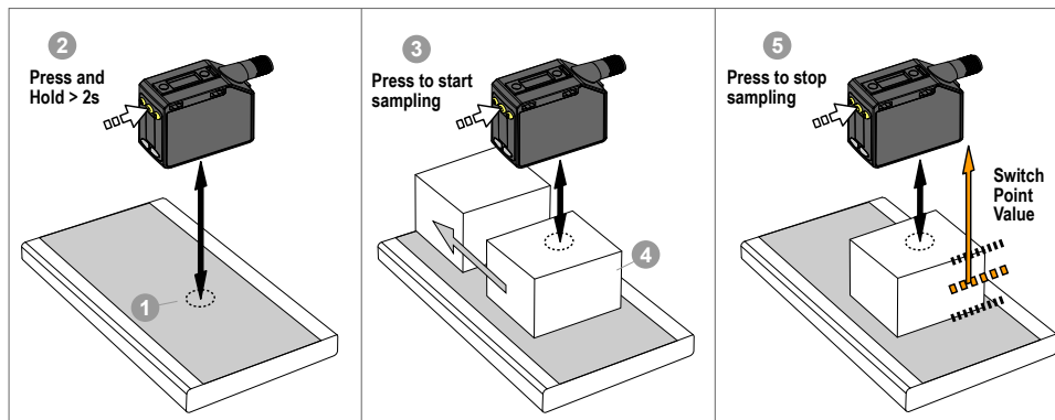
Figure 23. Dynamic Background Suppression
