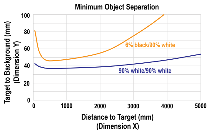
Figure 34. Minimum Object Separation for 5 ms Response Time
