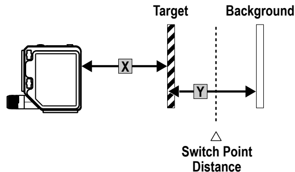
Figure 26. Minimum Object Separation Distance (90% to 6% reflectance) for the 2000 mm Models
