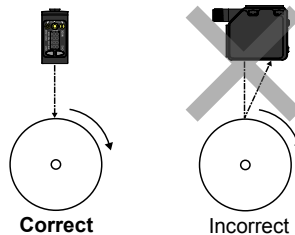
Figure 9. Orientation for highly reflective target 1
