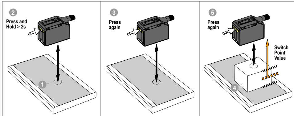
Figure 22. Two-Point Static Background Suppression (Light Operate shown)
