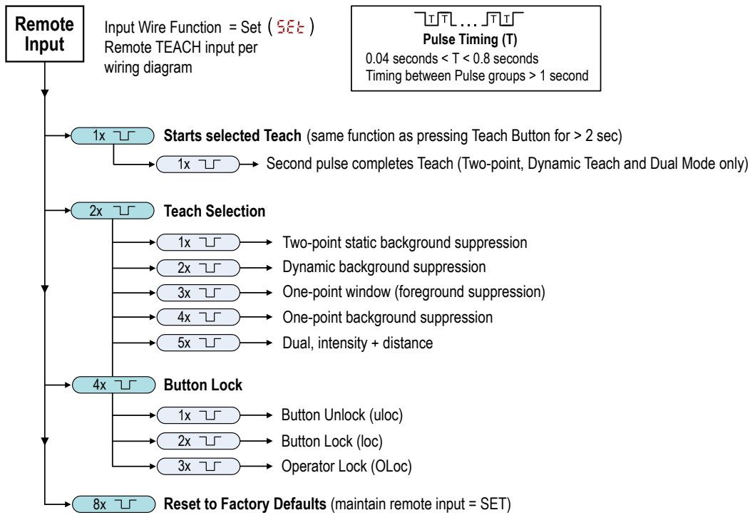
Figure 21. Remote Input Map
