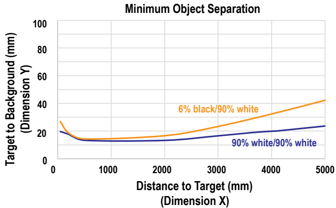
Figure 30. Minimum Object Separation for 50 ms Response Time
