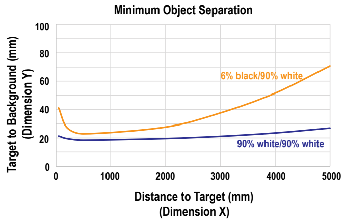
Figure 32. Minimum Object Separation for 15 ms Response Time
