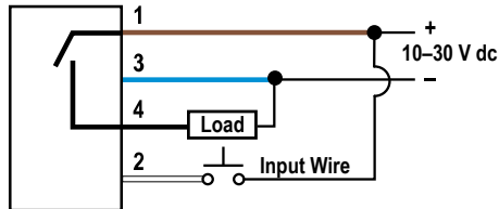
PNP Models
