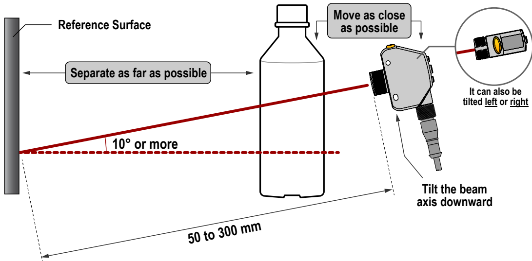
Figure 5. Mounting considerations
