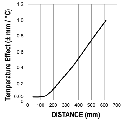
Figure 31. 610 mm Models
