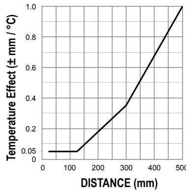
Figure 22. 500 mm Models
