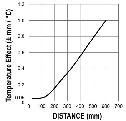
Figure 23. 600 mm Models
