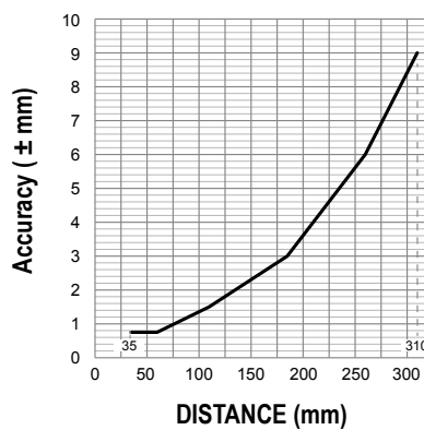
Figure 25. 310 mm Models
