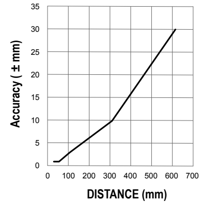
Figure 26. 610 mm Models
