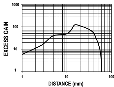
Figure 15. Excess Gain for Standard Sensitivity
