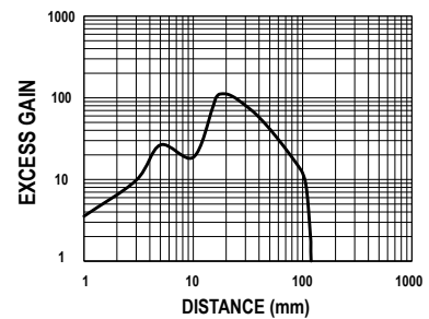
Figure 16. Excess Gain for Standard Sensitivity
