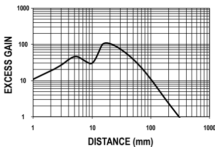
Figure 14. Excess Gain for Standard Sensitivity
