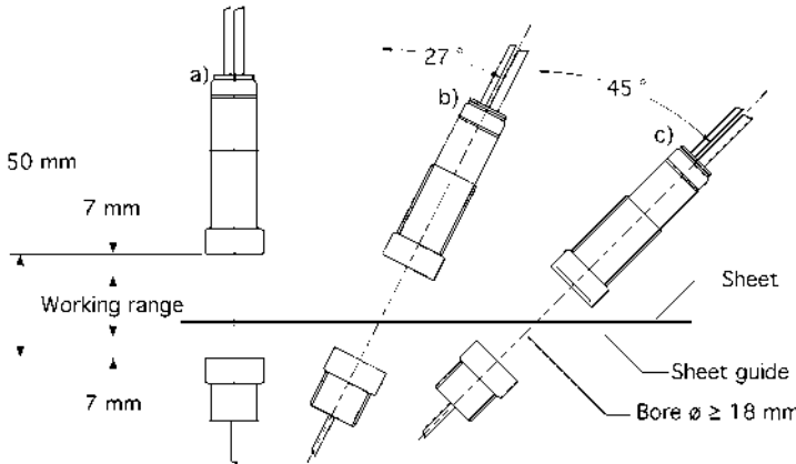
Fig. 1: Mounting and installation positions
