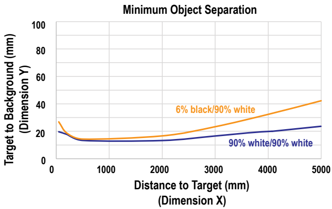
Figure 23. Minimum Object Separation for 50 ms Response Time
