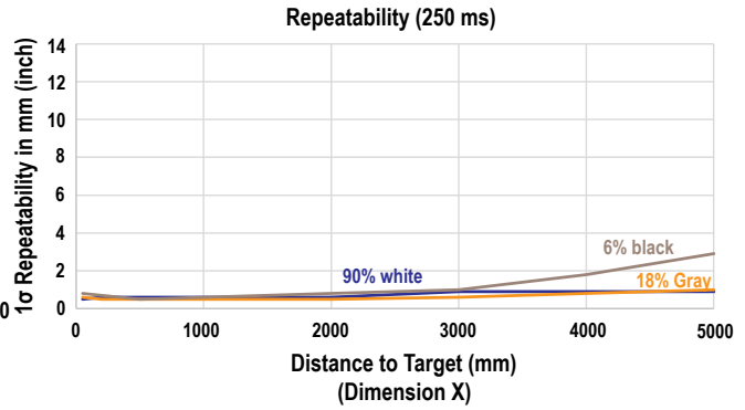
Figure 22. Repeatability for 250 ms Response Time
