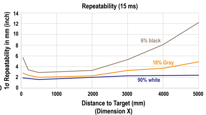
Figure 26. Repeatability for 15 ms Response Time
