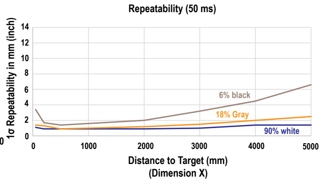
Figure 24. Repeatability for 50 ms Response Time
