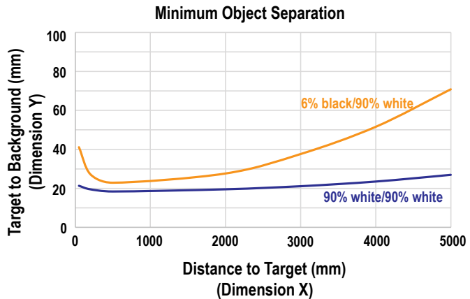
Figure 25. Minimum Object Separation for 15 ms Response Time
